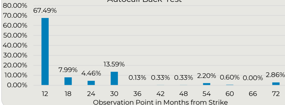
Autocall Back-Test
